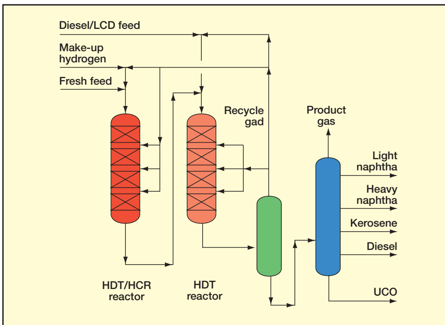
Figure 4 Split-feed injection
