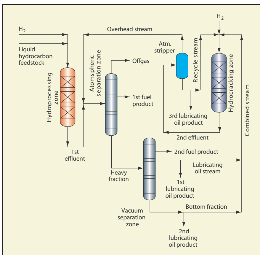
Figure 1 Isocracking for fuels and lubes
